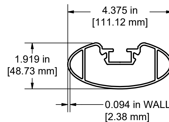
BOTTOM BAR MATERIAL - ALUMINUM
