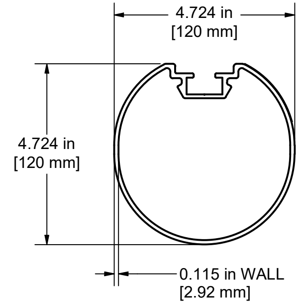
GOAL FRAME MATERIAL - ALUMINUM
