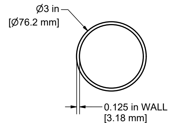
BACK POLE MATERIAL - ALUMINUM
