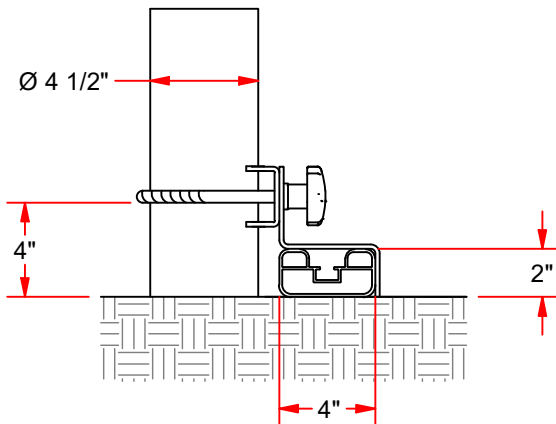
EXAMPLE INSTALLATION SIDE VIEW
